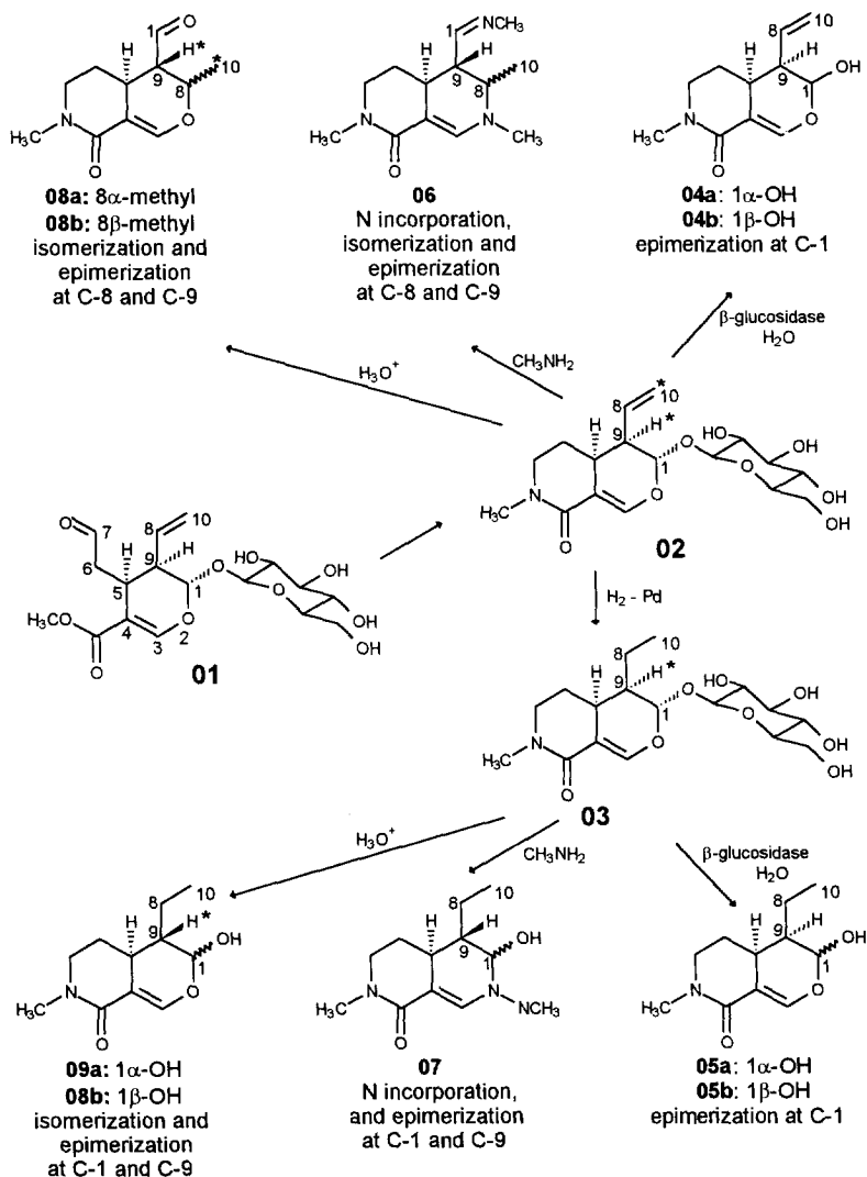
Scheme 1. Preparation and Deglycosylation of Secologanin Derivatives
