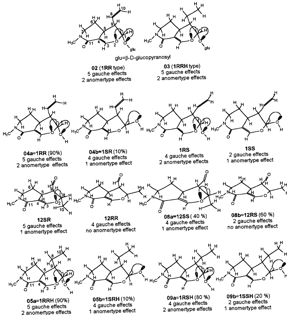
Scheme 2. Stereostructures of Educts and Products
