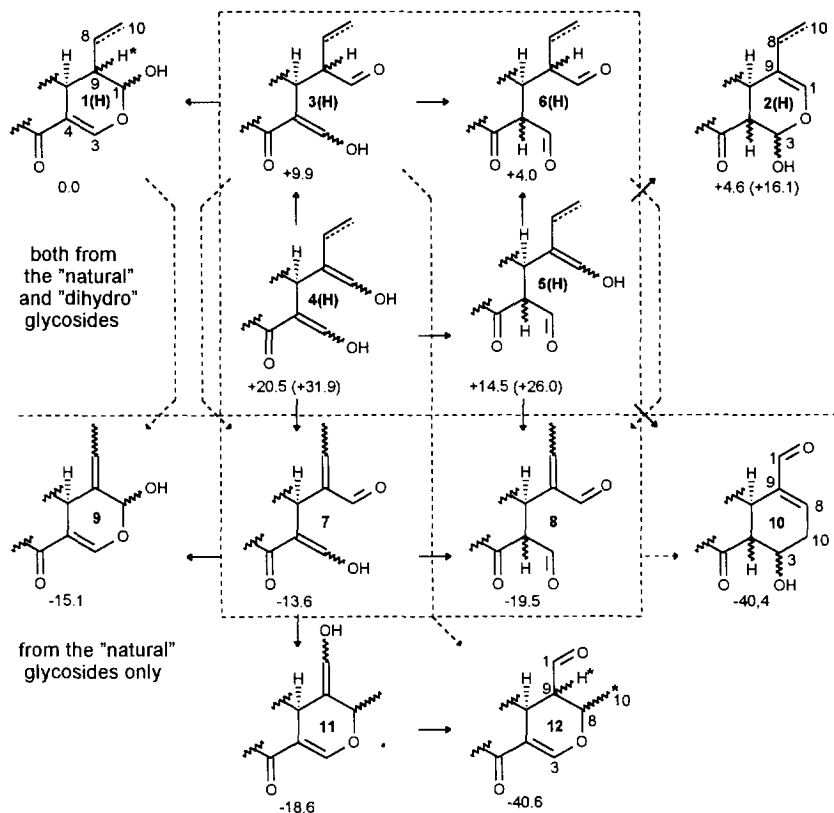
Scheme 3. The Energy Graph of the Possible Aglycones. Estimated relative free enthalpies of formation in kJ/mol. Energy values in parentheses conc possible aglycones derived from 8,10-dihydro glycosides.
