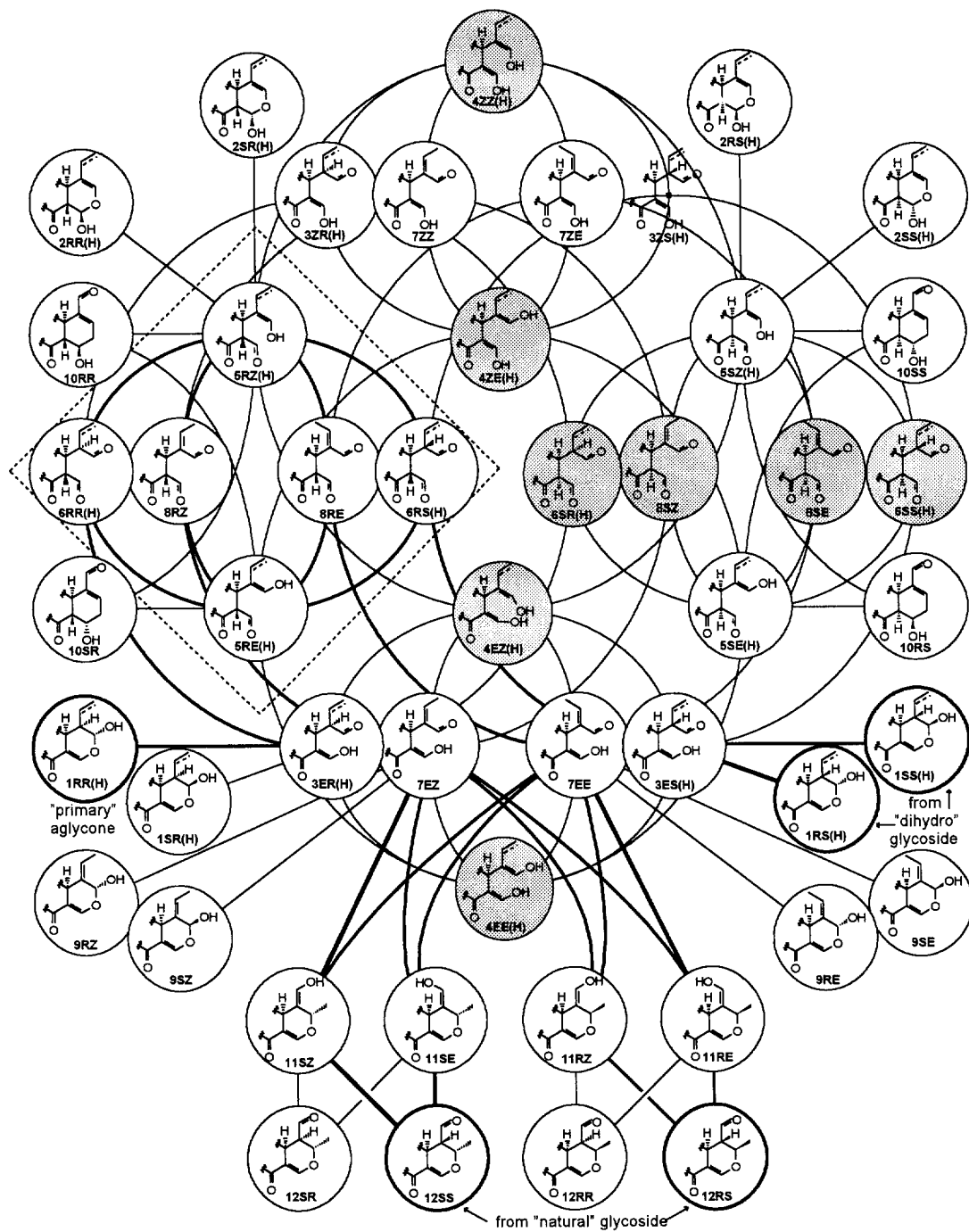
Scheme 5. Structure Graph of the Possible Aglycones
